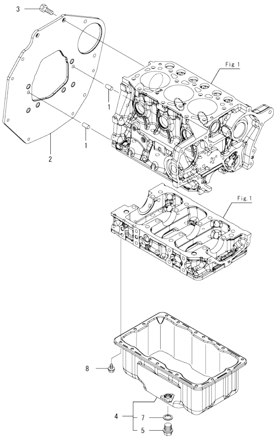
Fig.3. MOUNTING FLANGE & OIL SUMP
