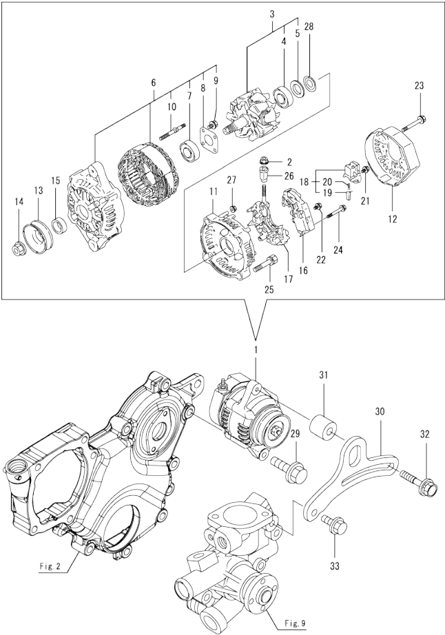
0CW10-M81502 ENGINE Fig.15. GENERATOR
