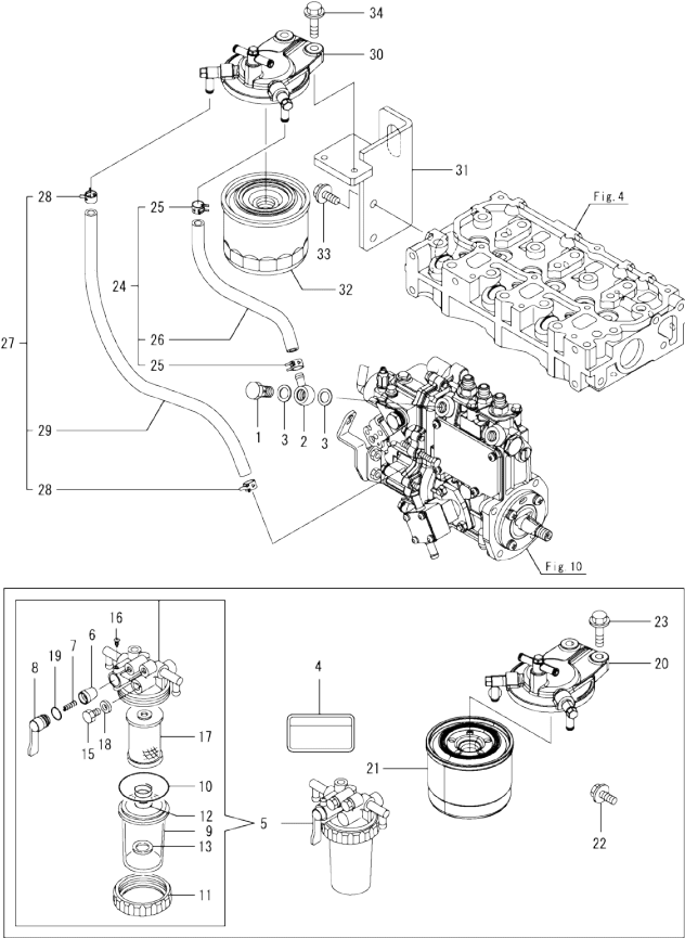
0CW10-M81502 ENGINE Fig.19. FUEL PIPE
