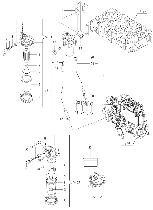
0CW10-M81502 ENGINE Fig.13. FUEL PIPE
